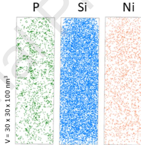
Figure 14. APT data of ion-irradiated (0.1 dpa, 300°C, @500 nm depth) Fe-9Cr-NiSiP alloys, see text and [112] for details.
