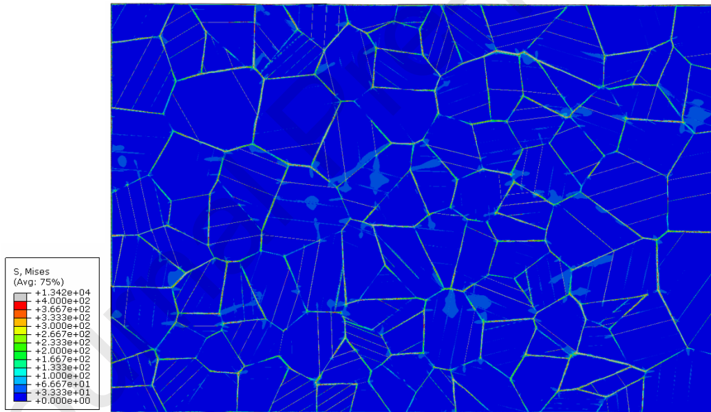
Figure 19. Mises stress [MPa] field of an aggregate containing 110 grains, with four channels per grain, stretched in the horizontal direction to \langle \epsilon_{11} \rangle = 0.01 [/]. Three slip systems activated in between the channels, one slip system activated in the slip channels. Channels are clearly visible.
