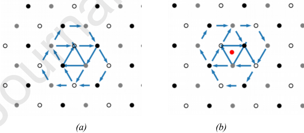
Figure 19. Easy (a) and hard (b) cores relaxed with DFTB in pure iron and in presence of C atoms respectively. In (b) we recover the reconstructed prismatic core identified by DFT in [154].
