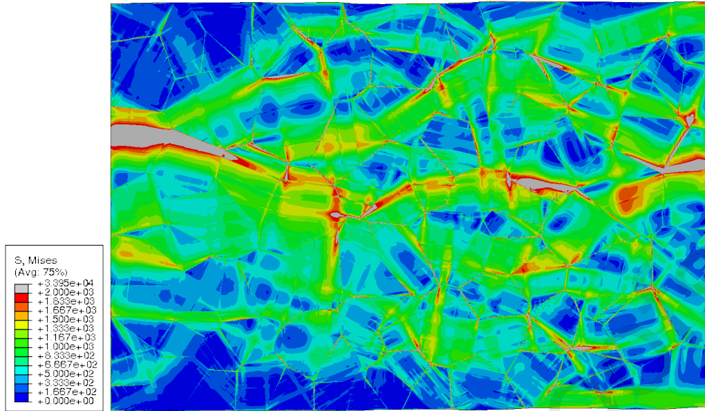
Figure 30. Mises stress [MPa] field of an aggregate containing 110 grains, with four channels per grain, stretched in the horizontal direction to \langle \epsilon_{11} \rangle = 0.01 [1]. One slip system activated in between the channels, one slip system activated in the slip channels.
