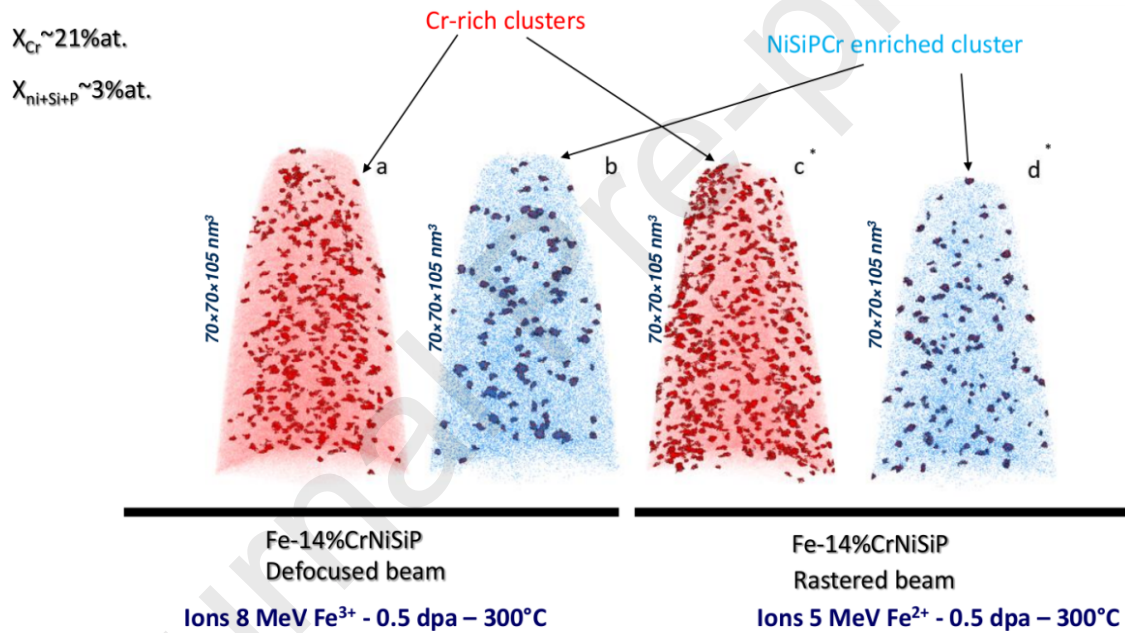
Figure 15: APT results for two different irradiation conditions: (left) 8 MeV Fe and defocused beam (right) 5 MeV Fe and rastered beam, both to 0.5 dpa.
