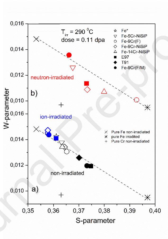
Figure 10. S versus W parameters of a) ion irradiated and b) neutron irradiated FeCr alloys and steels. The results are compared with existing data of similar materials and steels.
